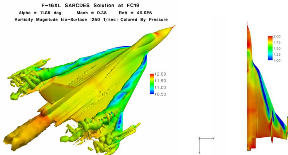
Figure 19: Flight Condition 19; a) iso-surfaces of vorticity magnitude colored by pressure, b) surface pressure coefficient distribution, C_p .
