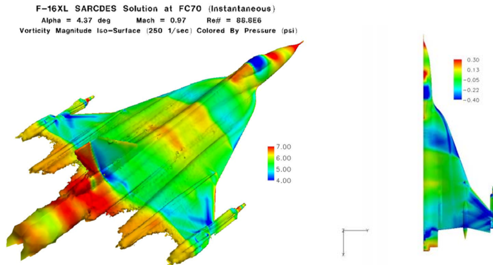
Figure 27: Flight Condition 70; iso-surfaces of vorticity magnitude colored by pressure, b) surface pressure coefficient distribution, C_p .
