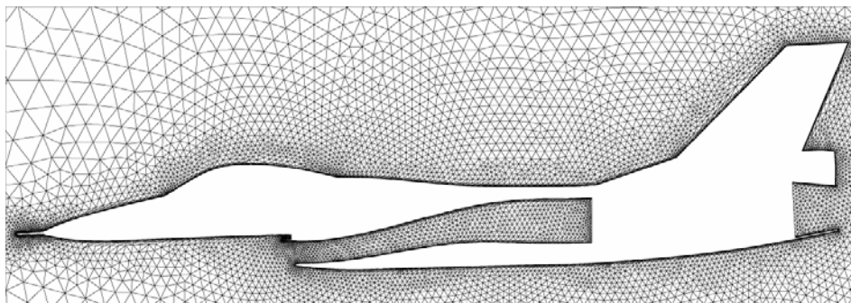
Figure 3: Symmetry plane of the F-16XL-1 baseline unstructured grid.
