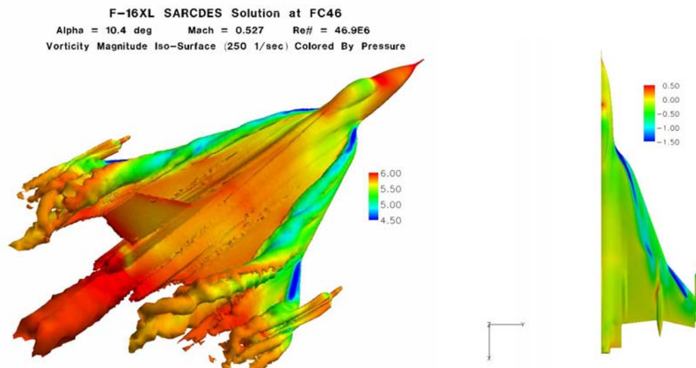
Figure 21: Flight condition 46; iso-surfaces of vorticity magnitude colored by pressure, b) surface pressure coefficient distribution, C_p .
