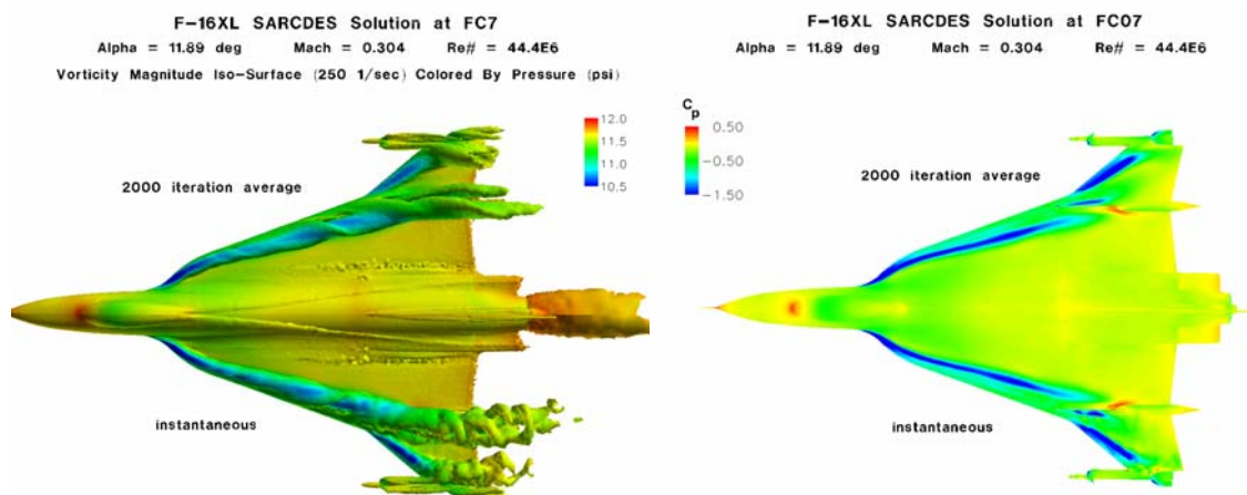
Figure 13: Comparison of an instantaneous solution to a solution time-averaged after 2000 time steps; a) iso-surfaces of vorticity magnitude colored by pressure, b) surface pressure coefficient distribution, C_p .
