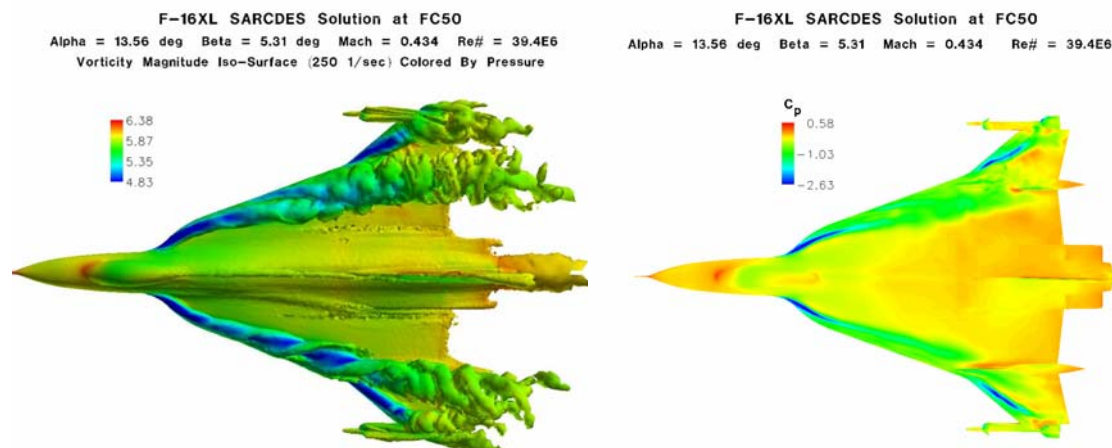
Figure 30: Flight Condition 50; iso-surfaces of vorticity magnitude colored by pressure, b) surface pressure coefficient distribution, C_p .
